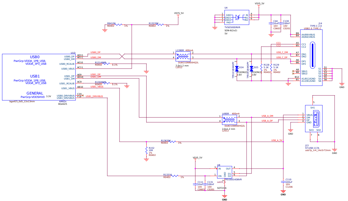
Fig. 3.5: USB-A and USB-C
